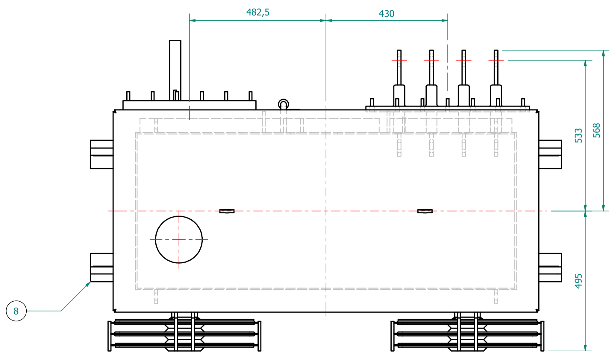
PLAN VIEW
